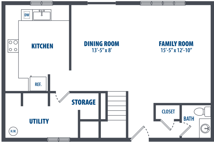
FIRST LEVEL
